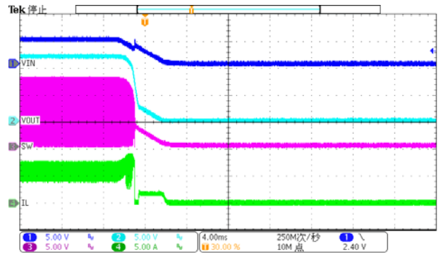
Figure 22. Power down(Iload=2A)
