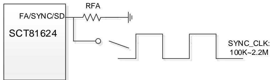
Figure16. Frequency Sync
