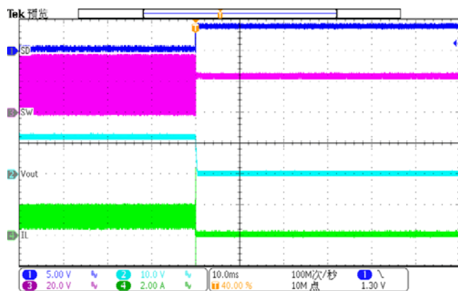
Figure 31. Shutdown entry
