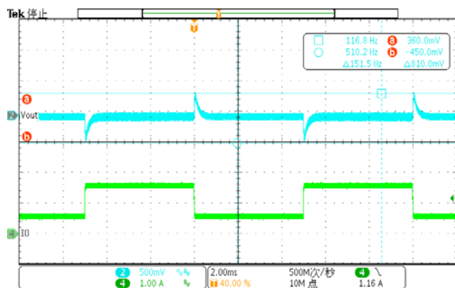
Figure 33. LoadTrans (Iload=0.5A-1.5A)
