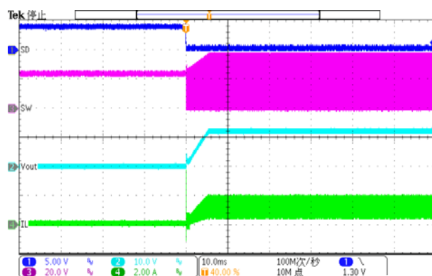
Figure 32. Shutdown remove
