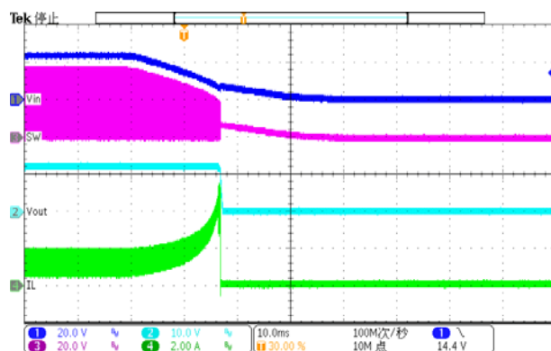
Figure 30. Power down(Iload=2A)
