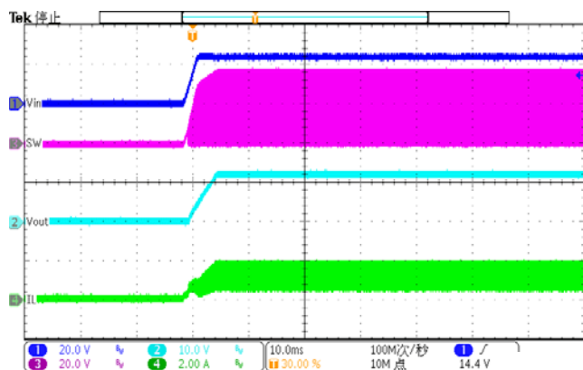
Figure 29. Power up(Iload=2A)
