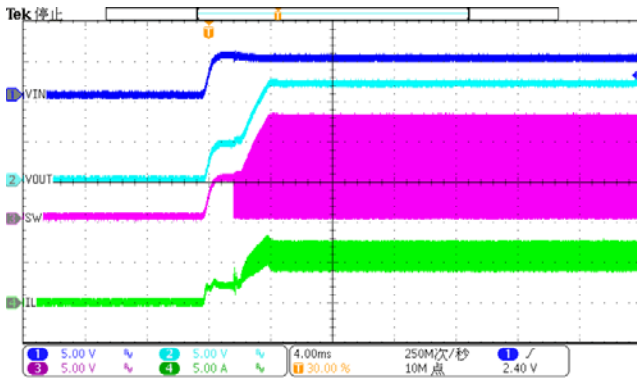
Figure 21. Power up(Iload=2A)
