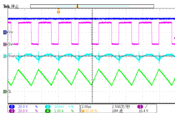
Figure 34. steady-state (Iload=2A)
