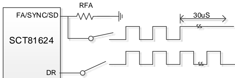
Figure18. Shutdown operation in Frequency Synchronization Mode
