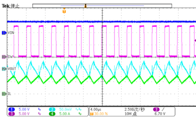
Figure 25. Steady-state (Iload=2A)
