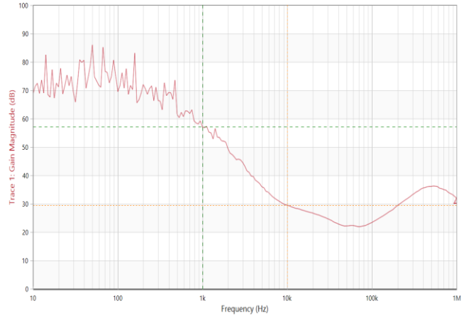
Figure 12. PSRR vs Frequency at Iout=100mA, Cout=4.7uF
