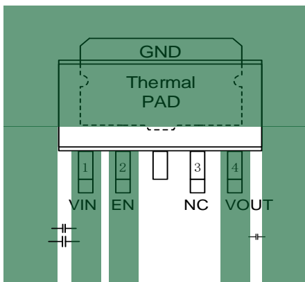
Figure 52. PCB Layout Example
