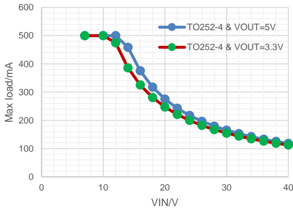
Figure 36. Maximum Output Current vs Input Voltage, TO252-4, T J ≤ 125°C(4-layer EVM)
