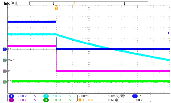
Figure 45. Disable (Iload=10mA)
