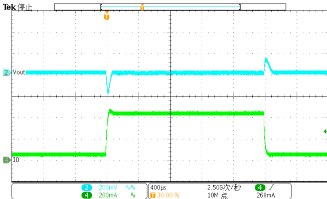
Figure 42. DC-DC Load Transient (50mA-450mA), VOUT=5V
