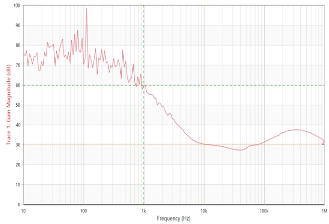
Figure 16. PSRR vs Frequency at Iout=100mA, Cout=22uF
