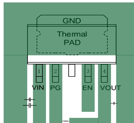
Figure 53. PCB Layout Example
