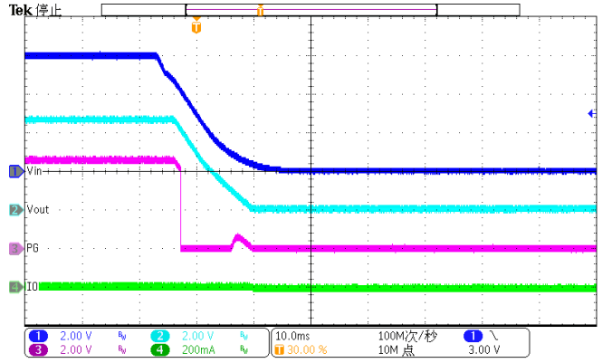
Figure 41. Slow Power down (Iload=10mA)
