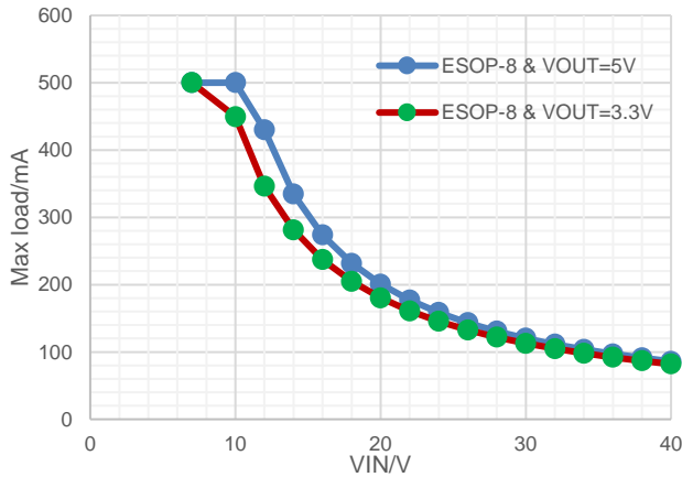
Figure 34. Maximum Output Current vs Input Voltage, ESOP-8, T J ≤ 125°C(4-layer EVM)
