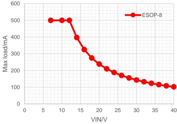
Figure 28. Maximum Output Current vs Input Voltage, VOUT=5V of ESOP-8, T_J \leq TSD\_R(2\text{-layer EVM})
