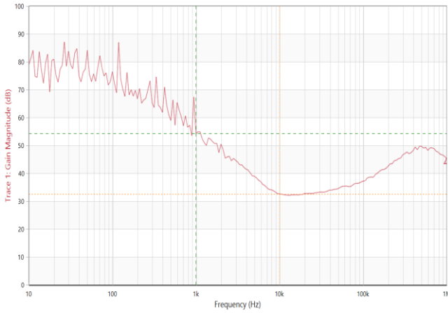
Figure 11. PSRR vs Frequency at Iout=10mA, Cout=4.7uF
