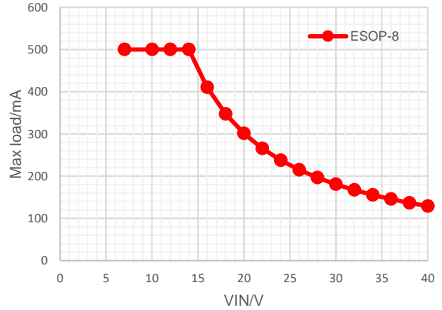
Figure 29. Maximum Output Current vs Input Voltage, VOUT=5V of ESOP-8, T_J \leq TSD\_R(4\text{-layer EVM})
