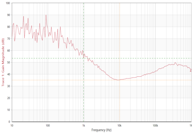
Figure 13. PSRR vs Frequency at Iout=10mA, Cout=10uF
