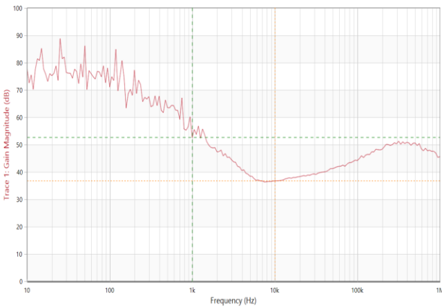
Figure 15. PSRR vs Frequency at Iout=10mA, Cout=22uF
