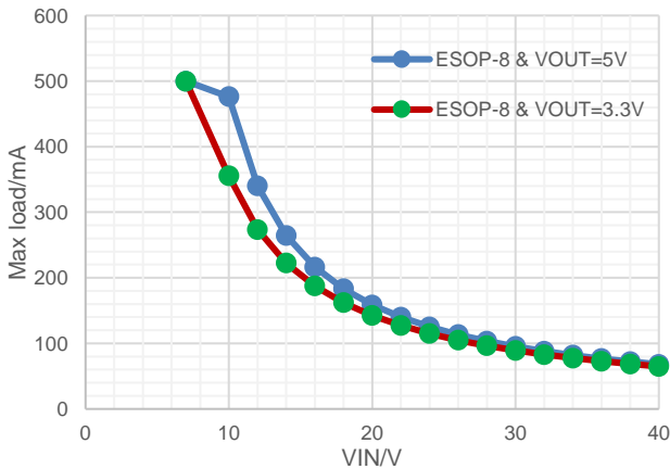
Figure 32. Maximum Output Current vs Input Voltage, ESOP-8, T_J \leq 125^\circ\text{C}(2\text{-layer EVM})
