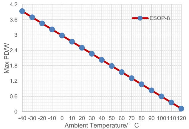
Figure 33. Maximum Allowed Power Dissipation vs Ambient Temperature, ESOP-8, T_J \leq 125^\circ\text{C}(2\text{-layer EVM})
