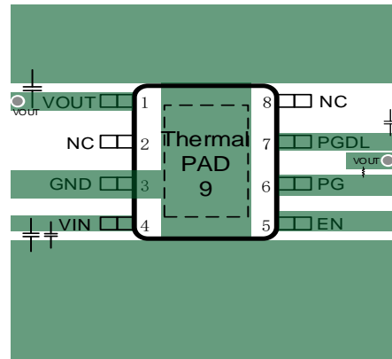
Figure 51. PCB Layout Example
