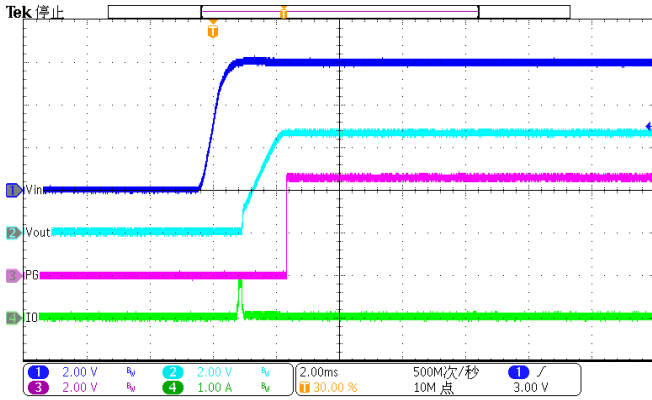
Figure 38. Power up (Iload=10mA)
