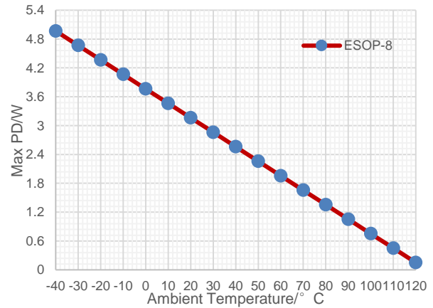
Figure 35. Maximum Allowed Power Dissipation vs Ambient Temperature, ESOP-8, T J ≤ 125°C(4-layer EVM)
