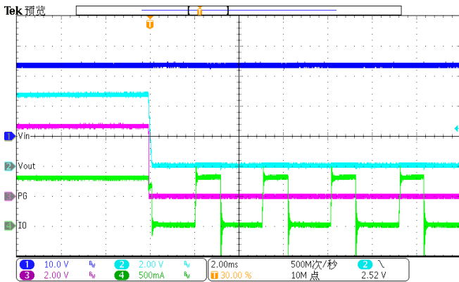
Figure 48. Enter Over Temperature Protection(Vin=24V)
