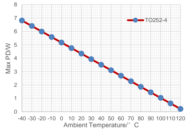
Figure 37. Maximum Allowed Power Dissipation vs Ambient Temperature, TO252-4, T J ≤ 125°C(4-layer EVM)
