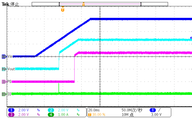
Figure 40. Slow Power up (Iload=10mA)
