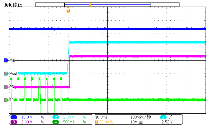
Figure 49. Exit Over Temperature Protection(Vin=24V)
