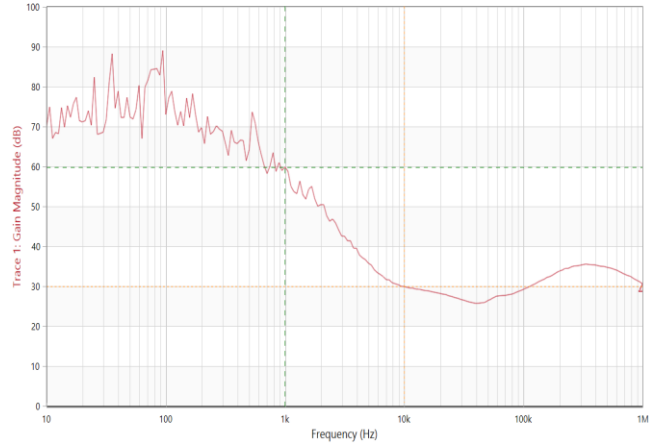
Figure 14. PSRR vs Frequency at Iout=100mA, Cout=10uF
