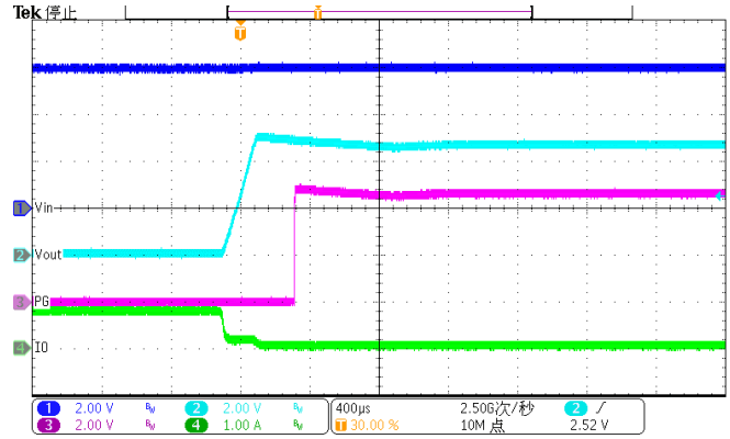
Figure 47. Exit Over Current Protection (Iload=1A)
