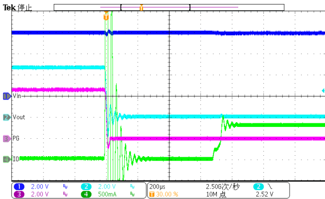
Figure 46. Enter Over Current Protection (Iload=1A)
