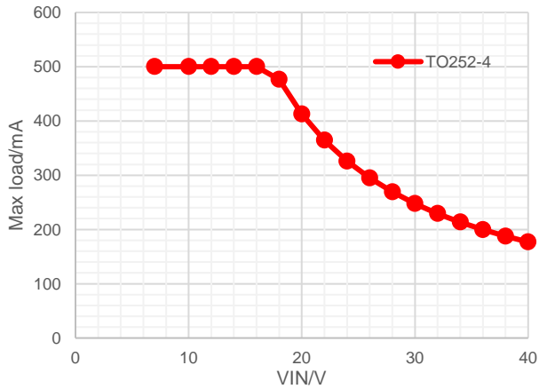
Figure 30. Maximum Output Current vs Input Voltage, VOUT=5V of TO252-4, T_J \leq TSD\_R(4\text{-layer EVM})
