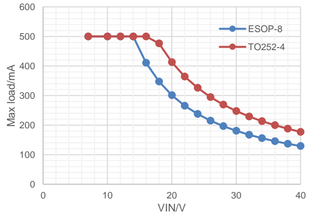
Figure 31. Maximum Output Current vs Input Voltage, VOUT=5V of Different Packages, T_J \leq TSD\_R(4\text{-layer EVM})
