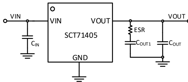
Figure 26. SCT71405 Typical Application Schematic with Large Output Capacitor
