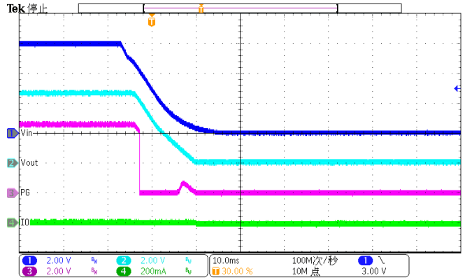
Figure 39. Power down (Iload=10mA)
