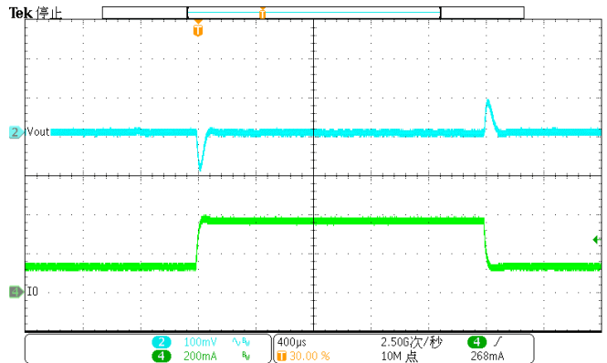
Figure 43. DC-DC Load Transient (130mA-370mA), VOUT=5V
