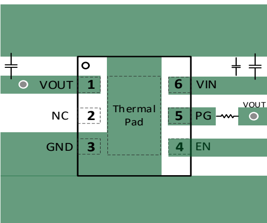
Figure 47. PCB Layout Example
