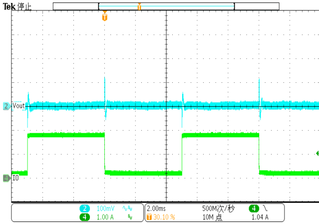
Figure 23. DC-DC Load Transient (0.2A-1.8A, 1.6A/us)
