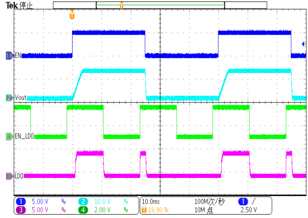
Figure 32. EN/ EN_LDO toggle (Iout=1A, Ildo=0.1A)
