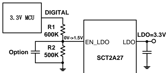
Figure 10. 3.3V Digital signal set 3.3V LDO output,
