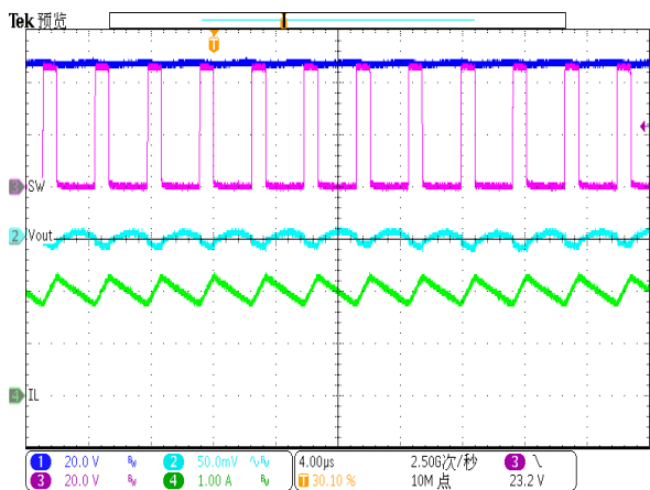
Figure 27. DC-DC Output Ripple (Iload=2A)
