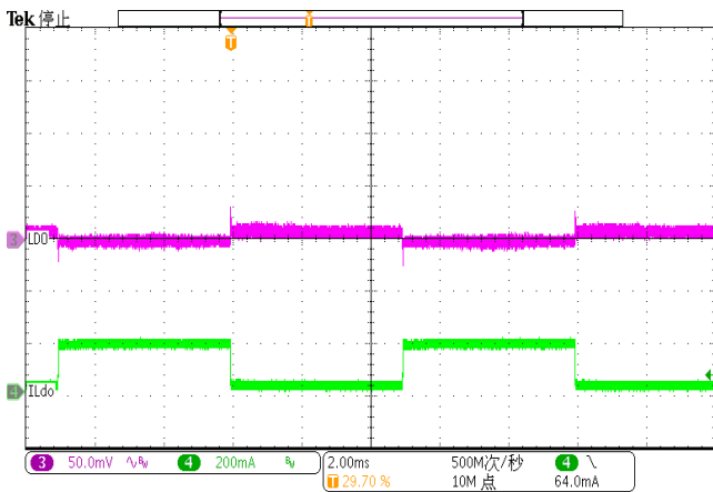
Figure 33. Load Transient (0.02A-0.18A, 1.6A/us)
