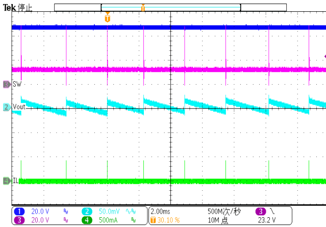
Figure 25. DC-DC Output Ripple (Iload=0A)
