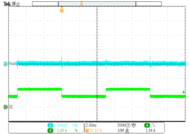
Figure 24. DC-DC Load Transient (0.75A-1.25A, 1.6A/us)
