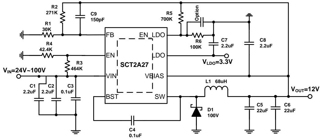
Figure 16. SCT2A27 Design Example, BUCK 12V Output , LDO 3.3V Output
