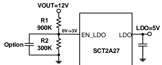
Figure 15. Resistor divider set 5V LDO output
