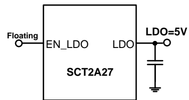
Figure 13. Float EN_LDO set 5V LDO output
