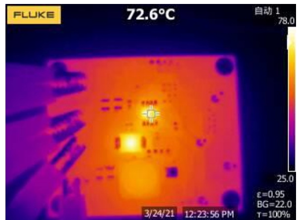
Figure 28. Thermal, 48VIN, 12Vout, 2A
