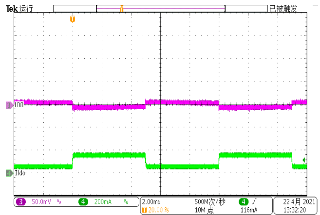
Figure 34. Load Transient (0.05A-0.15A, 1.6A/us)
