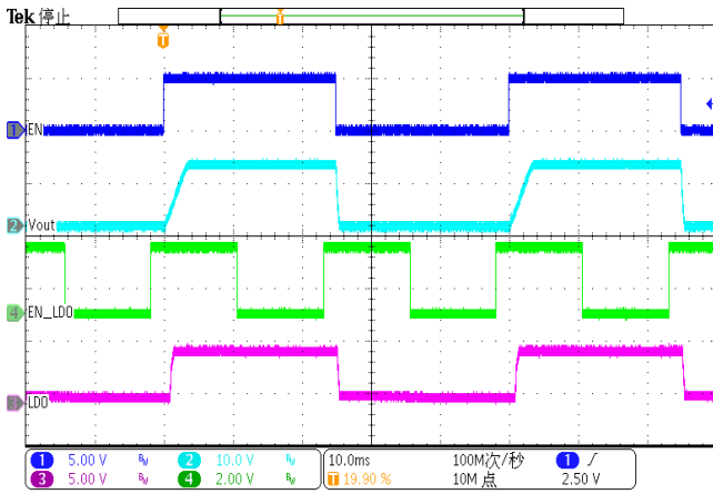
Figure 31. EN/ EN_LDO toggle (Iout=1A, Ildo=0A)
