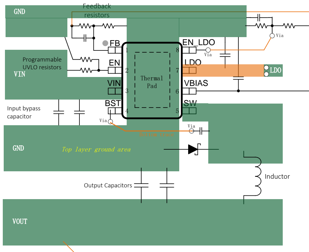
Figure 35. PCB Layout Example
