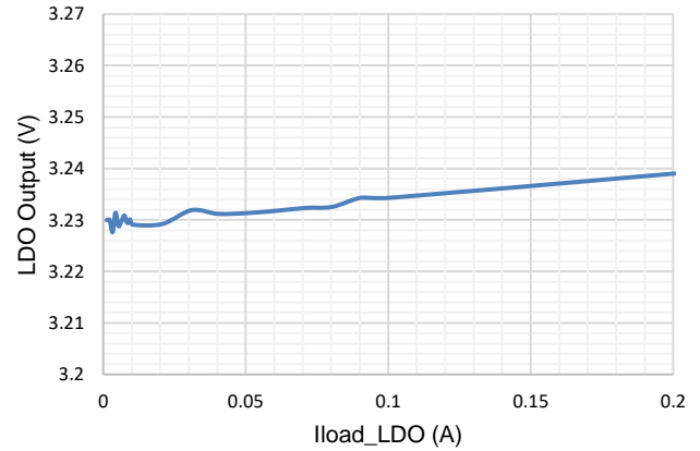
Figure 5. LDO Load Regulation, LDO output 3.3V
