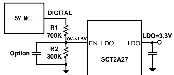
Figure 11. 5V Digital signal set 3.3V LDO output
