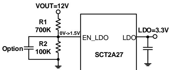
Figure 14. Resistor divider set 3.3V LDO output
