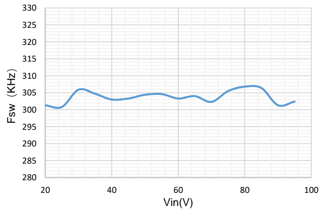
Figure 7. Switching Frequency vs Vin, Vout=12V
