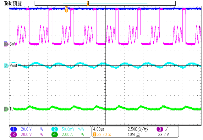
Figure 26. DC-DC Output Ripple (Iload=0.1A)
