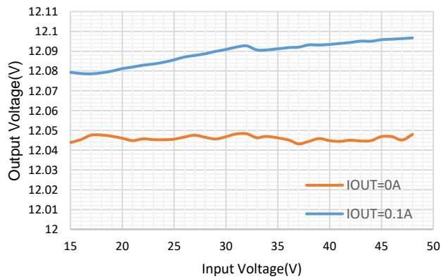
Figure 6. Line Regulation
