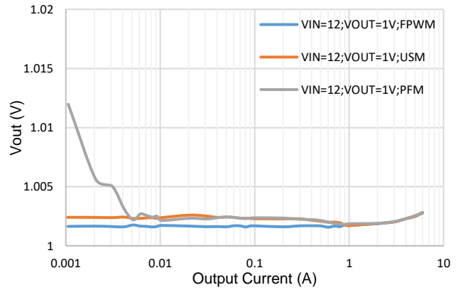
Figure 5. Load Regulation, Vout=1V, fsw=800kHz
