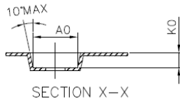
SECTION X-X
